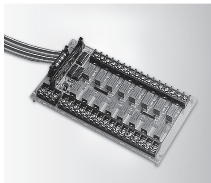
PCLD-885
