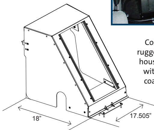
C-VS-1800-ECO shown with optional video system (PT-VIDEO-4) for prisoner transport compartments.
