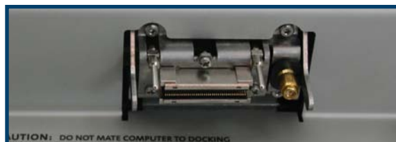
CAUTION: DO NOT MATE COMPUTER TO DOCKING Docking Head Connector shown in the activated 'DOCK' position without a docked computer in place.
