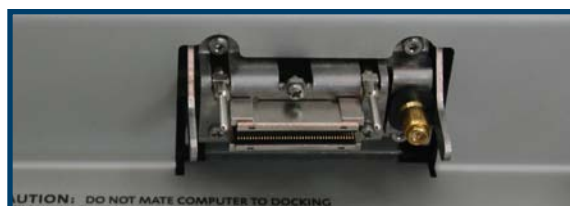
CAUTION: DO NOT MATE COMPUTER TO DOCKING Docking Head Connector shown in the activated 'DOCK' position without a docked computer in place.
