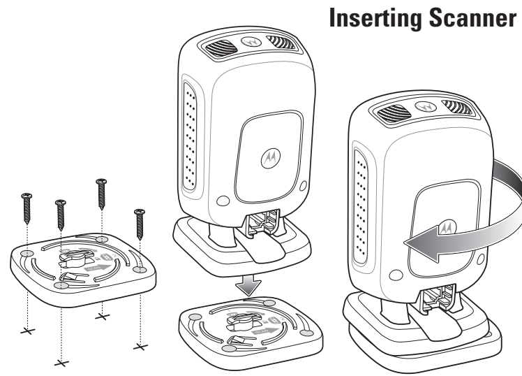
Inserting Scanner
