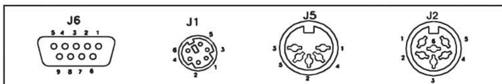
CONNECTOR ARRANGEMENT
